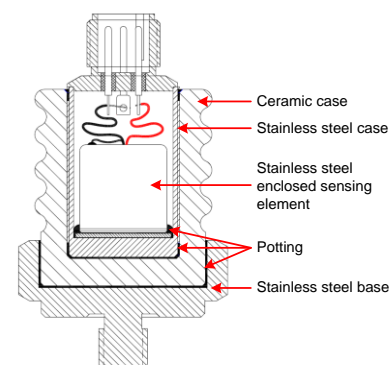
Figure 1: internal components
