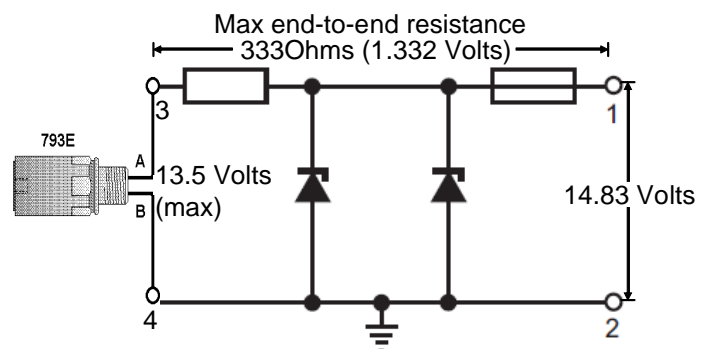
Figure 3.1.1.2 - Circuit voltages
