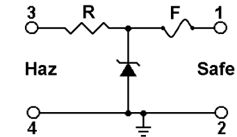
Figure 2.2.1 - Basic zener barrier schematic
