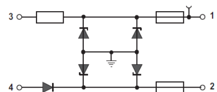
Figure 3.2.1.1 – ISBS-STD-06 schematic
