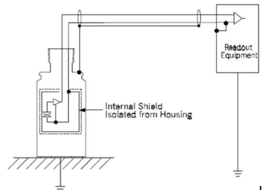
Figure 5b: A properly grounded installation
