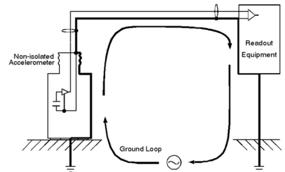
Figure 5a: A poorly grounded installation
