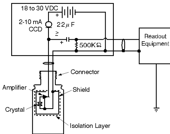
Figure 3: Schematic of a sensor power supply
