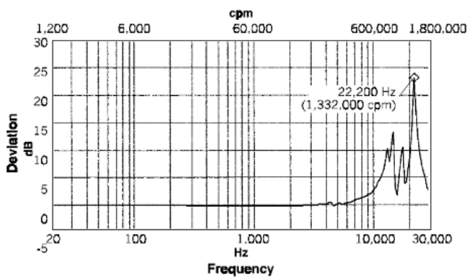
Figure 8c: QuickLINK™ mounting resonance
