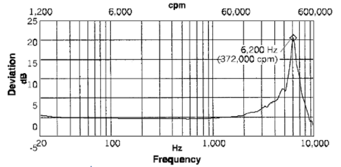
Figure 8b: Magnet mounting resonance
