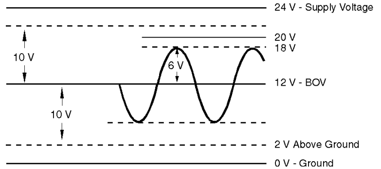
Figure 2: AC signal limits
