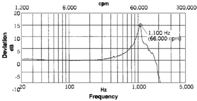
Figure 8a: Probe tip mounting resonance
