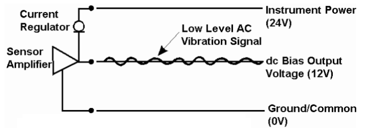
Figure 1: Sensor amplifier circuits
