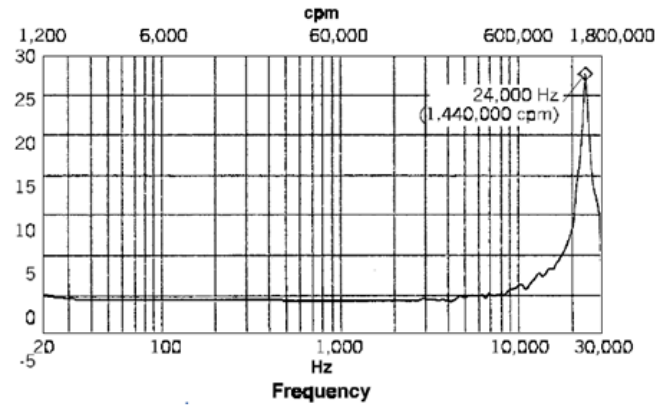
Figure 8d: Stud mounting resonance
