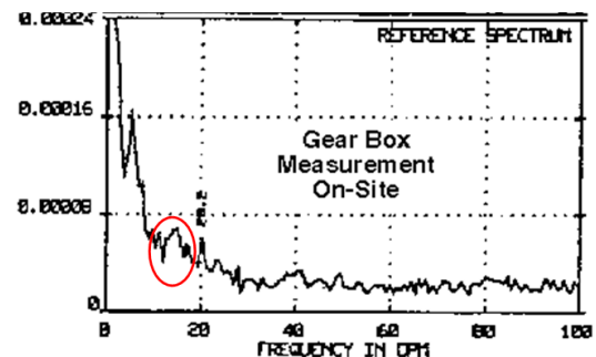
Figure 7: Ski-slope noise caused by analog integration
