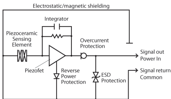
Figure 2: Circuit diagram for a PVT
