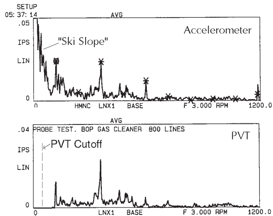
Figure 5: Spectral plot comparison of an accelerometer and a PVT
