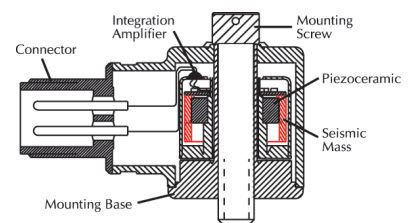
Figure 1b: Shear mode PVT
