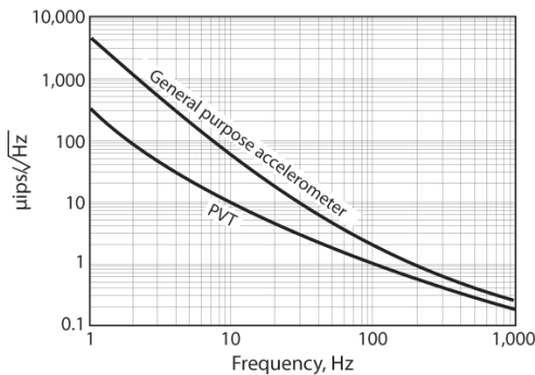
Figure 4: Noise response comparison between a 100 mV/g accelerometer and a 100 mV/g PVT, normalized in terms of velocity
