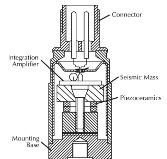
Figure 1a: Compression mode PVT
